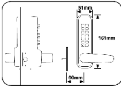
Model 410/415 With deadlocking tubular latchbolt
